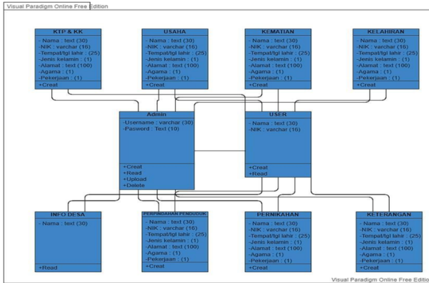
Gambar 4 Class Diagram
