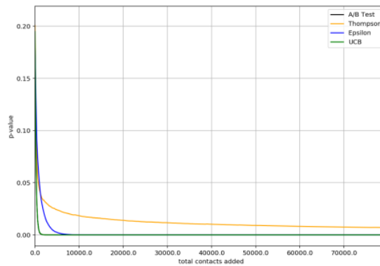
1 Figure 16. Statistical significance for high-difference 2-variant simulations
