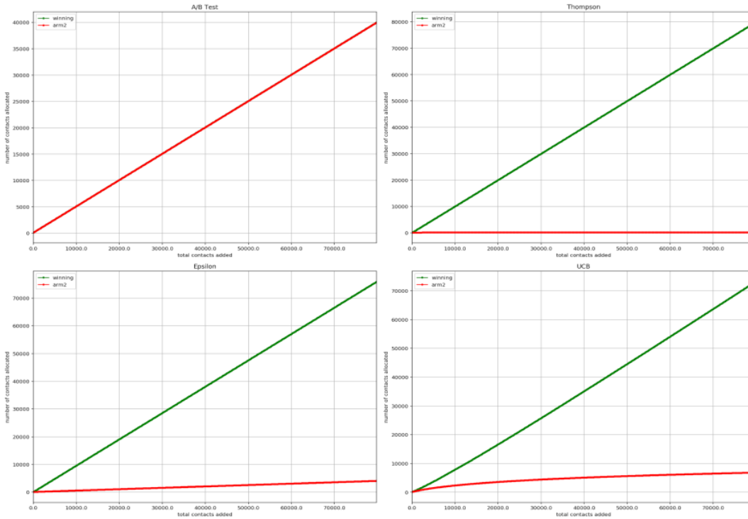
Fig. 10. Average interaction allocations from two-variant high-difference simulations
