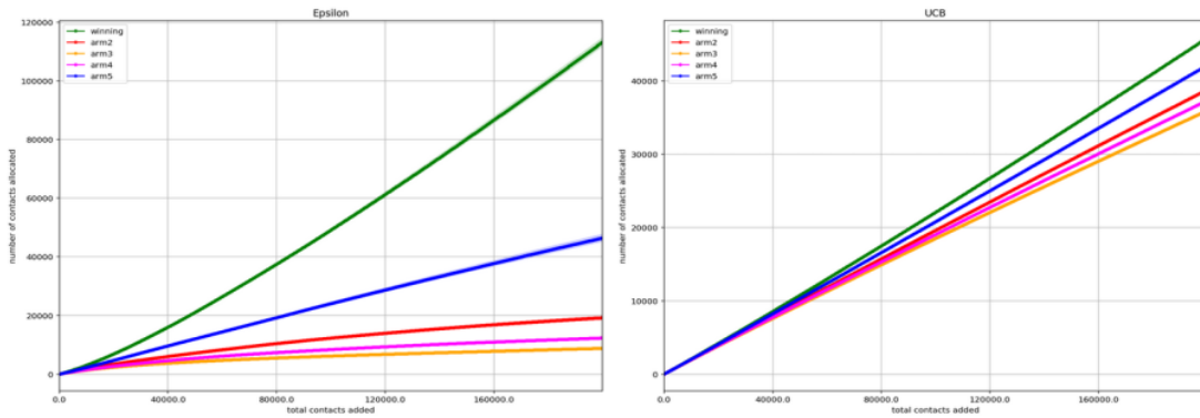
Fig. 6. Low-Difference Conversion Rate Simulation's average communication allocation
