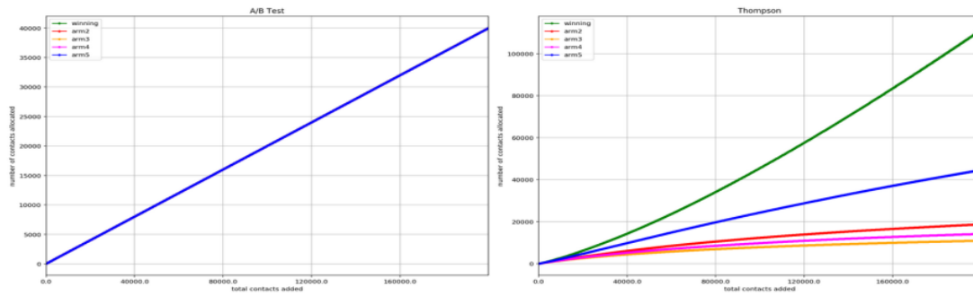
Fig. 5. A/B and Thompson Sampling testing
