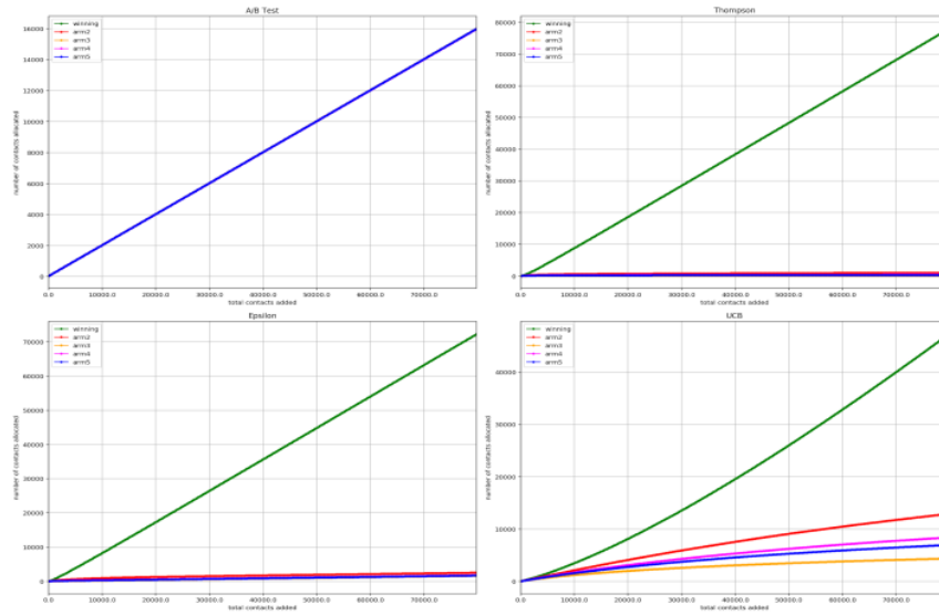
1 Fig. 9. Average contact allocations from high-difference conversion rate simulations
