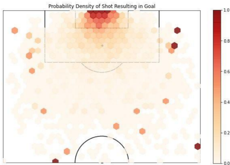
Fig. 7. Probability Density of Shot Resulting in Goal
