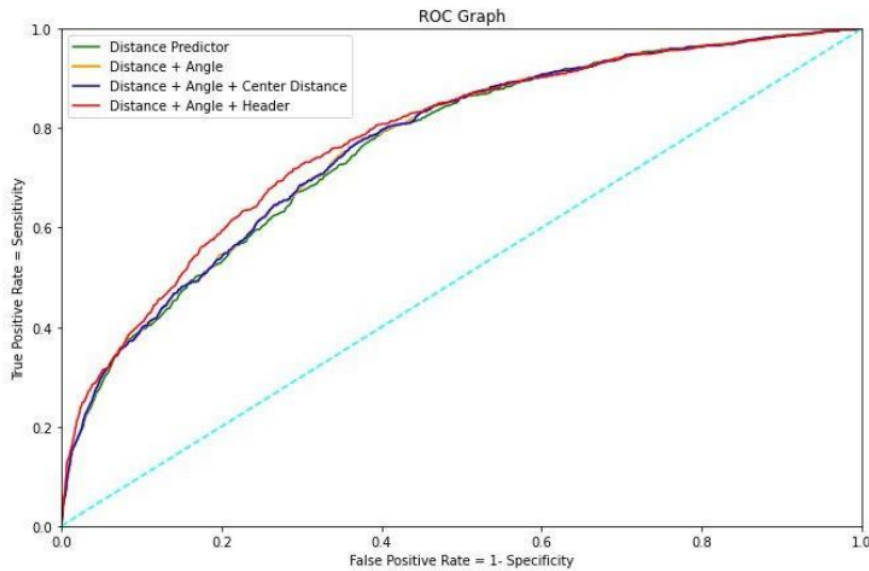
Fig. 22. ROC Model for Distance Predictor
