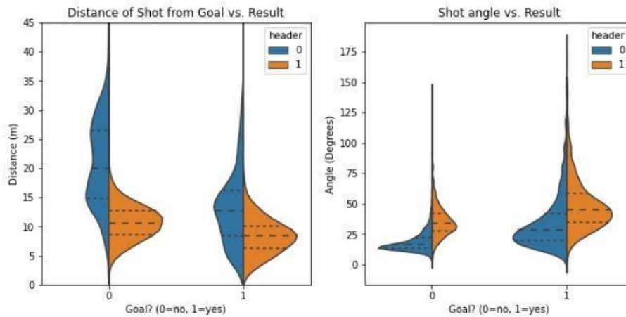
Fig. 5. Shot Distance Comparison
