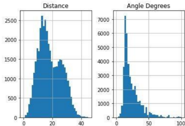
Fig. 3. Distributions of Shots by Distance and Angle
