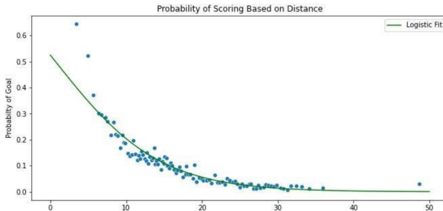
Fig. 16. Probability of Scoring Based on Distance
