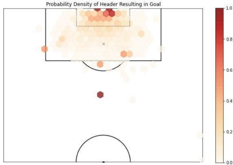
Fig. 8. Probability Density of Header Resulting in Goal
