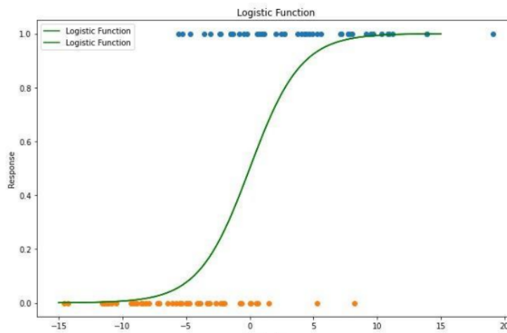
Fig. 14. Logistic Function
