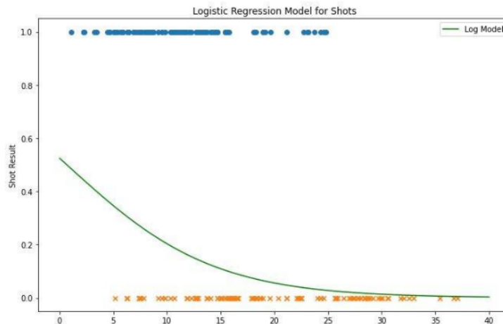
Fig. 15. Logistic Regression Model for Shots
