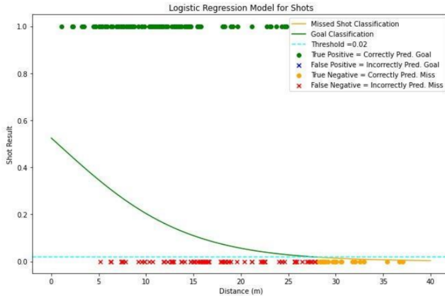
Fig. 19. Logistic Regression Model for Shots
