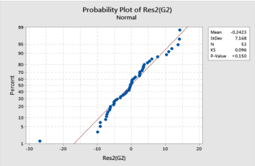
9 Figure B.6. Residual normality test results of the ARIMA residual model.
