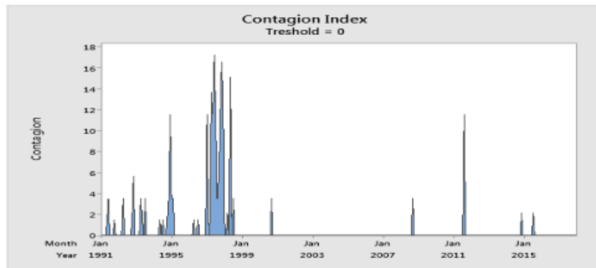
Gambar 5.10: Contagion Index
