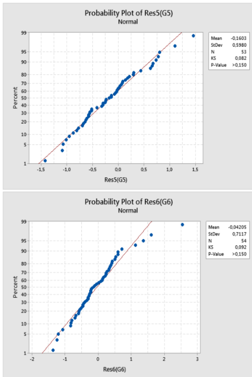
Gambar 5.8 Hasil Uji Normalitas ARIMA Residual Model
